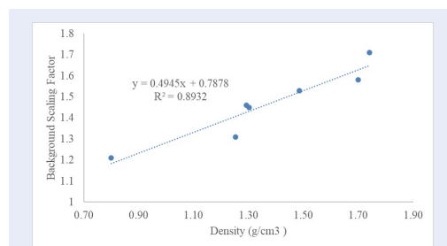
Figure 2: Correlation between the fitted background scaling factor ( b ) and the bulk density of the analyzed samples.
