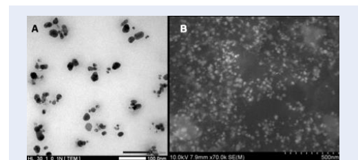
Figure 7: Morphology of biosynthesized silver nanoparticles at the 1-hour reaction time: (A) transmission electron micrograph; (B) scanning electron micrograph.
